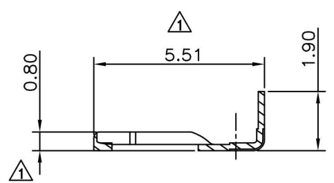
B-B SEC
