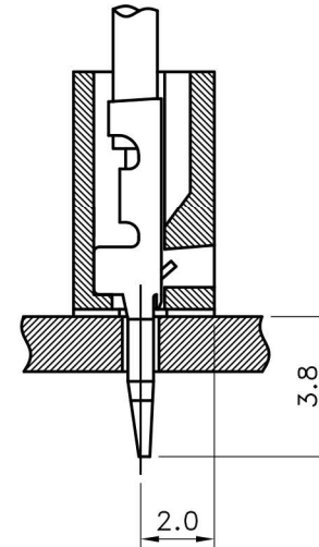
Mated Drawing (REF.)
