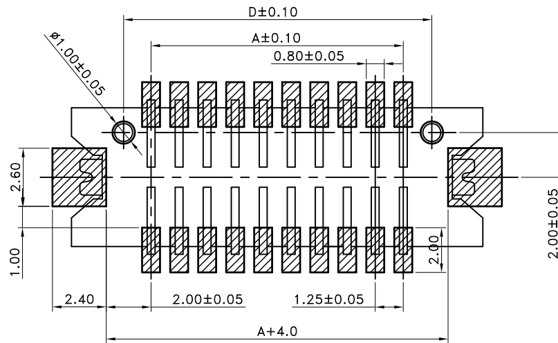
△14 Recommended P.C.B. Layout
